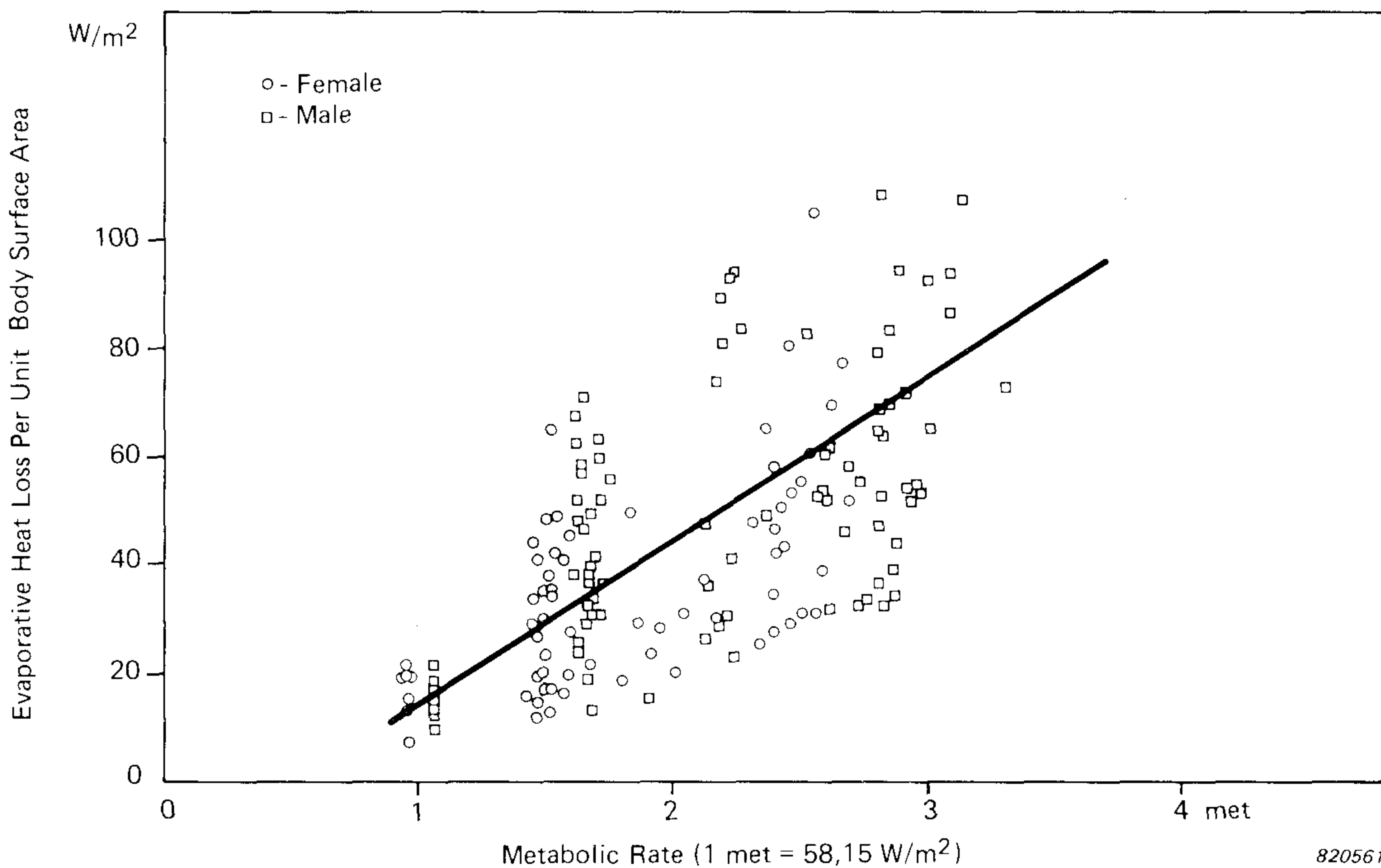
Fig. 3. Evaporative heat loss as a function of the activity level for persons in thermal comfort. In order to maintain thermal comfort the ambient temperature is lower the higher the activity level [2]
