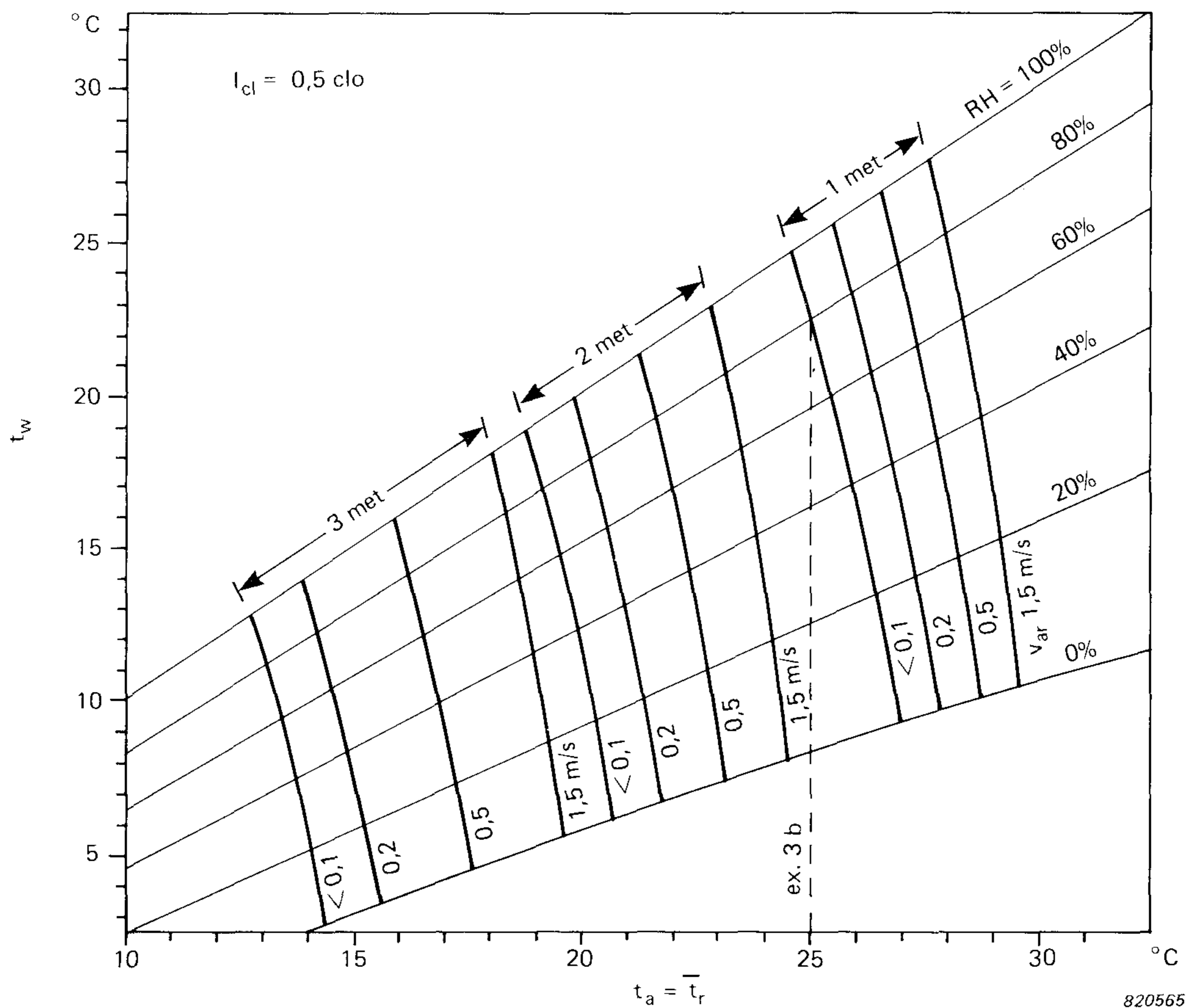
Fig. 7. Comfort lines for 0,5 clo. Wet bulb temperature t_w as a function of air temperature t_a = \text{mean radiant temperature } \bar{t}_r for various relative velocity v_{ar} and activity M as parameters
