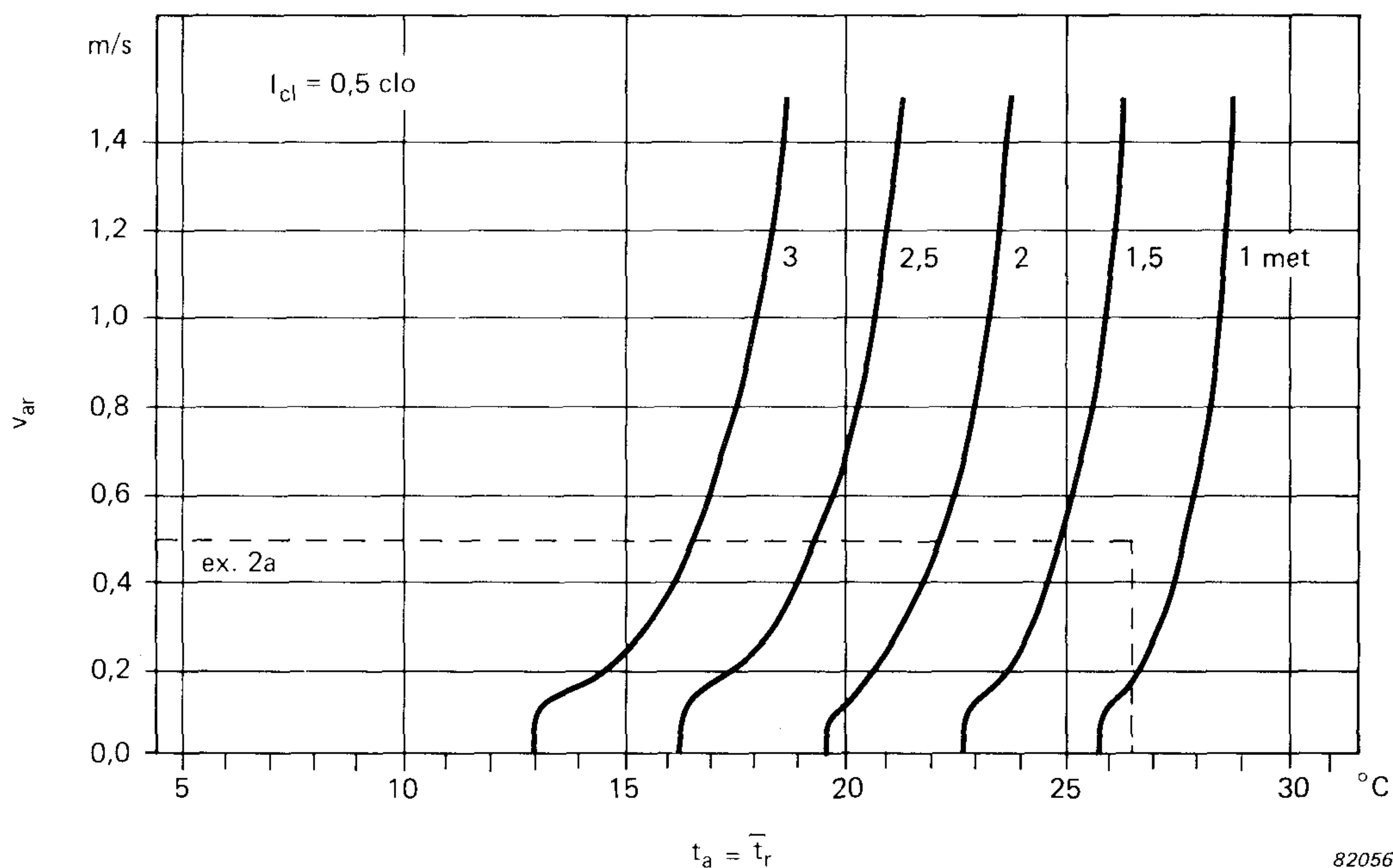
Fig. 4. Comfort lines for 0,5 clo and Relative Humidity 50%. Relative Velocity v_{ar} as a function of air temperature t_a = \text{mean radiant temperature}, \bar{t}_r for various activity M as parameter
